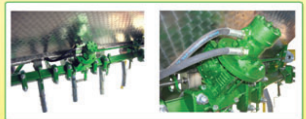
Trasmissione idraulica per spandiconcime, sarchiatrici, interruttori concime e insolcatrici Hydraulic transmission for fertilizer spreaders, hoeing machines, fertilizer coulters openers and furrow machines
